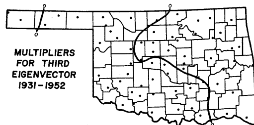
FIGURE 9. Multipliers for third eigenvector, 1931-1952.
